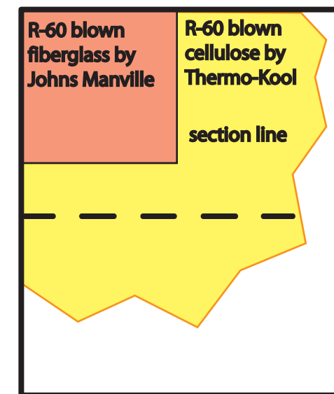
Roof Insulation Test Section plan view - not to scale
